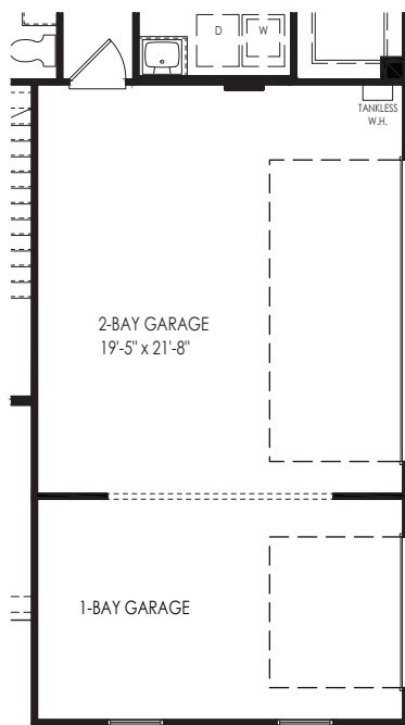
3-CAR SIDE ENTRY
