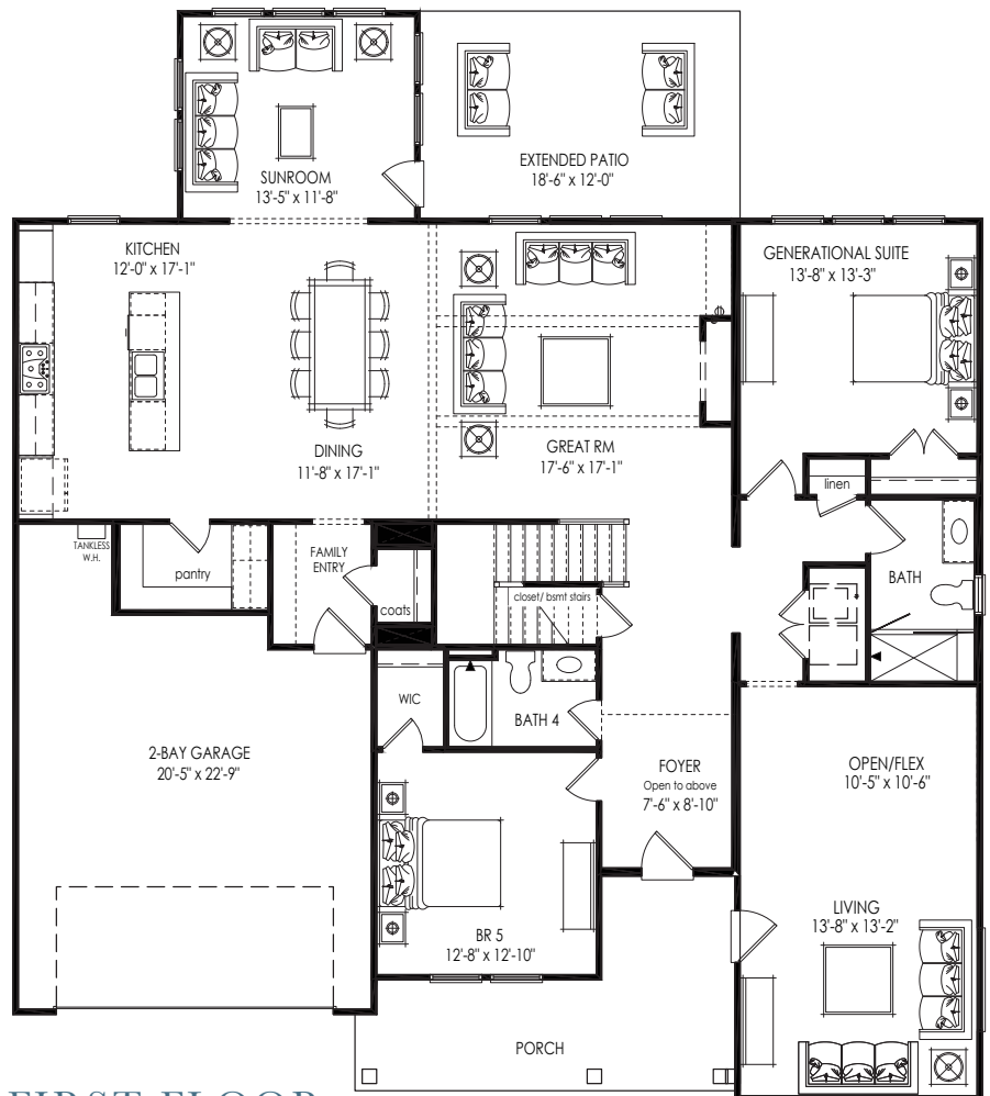
FIRST FLOOR
