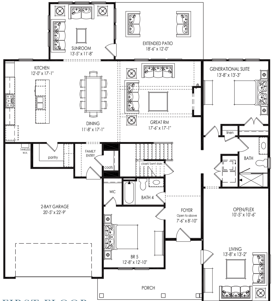
FIRST FLOOR
