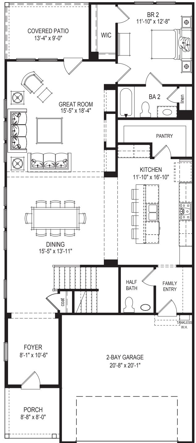
FIRST FLOOR
