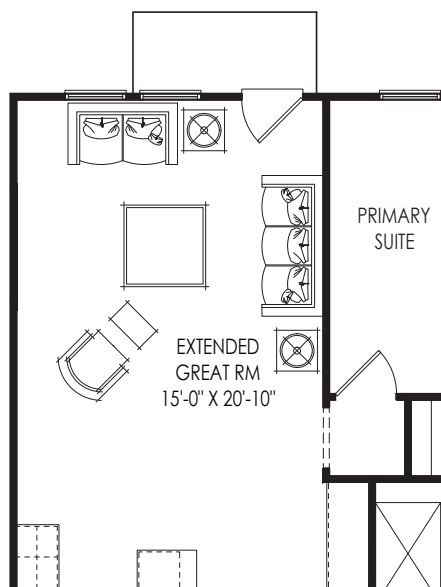
EXTENDED GREAT ROOM OPTION
